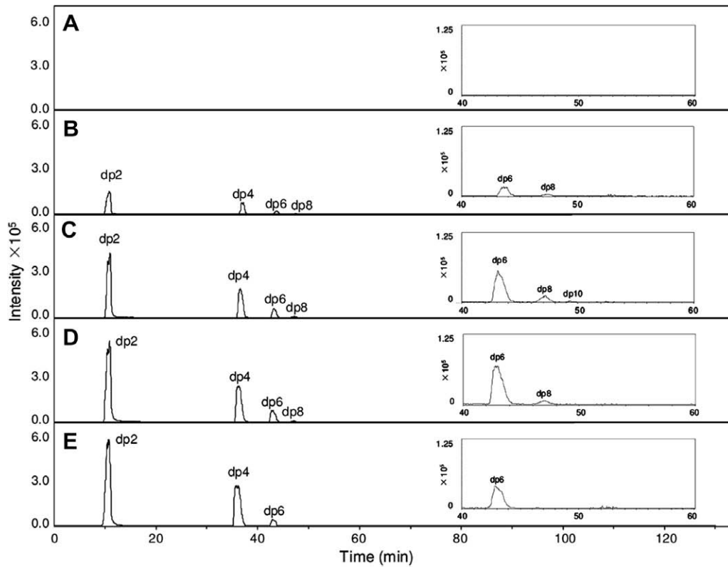
Fig. 2. EIC of products digested by chondroitinase ABC ( P. vulgaris ): (A) 0-min aliquots; (B) 10-min aliquots; (C) 30-min aliquots; (D) 60-min aliquots; (E) 120-min aliquots. Insets are 5× intensity magnification of 40 to 60 min.
