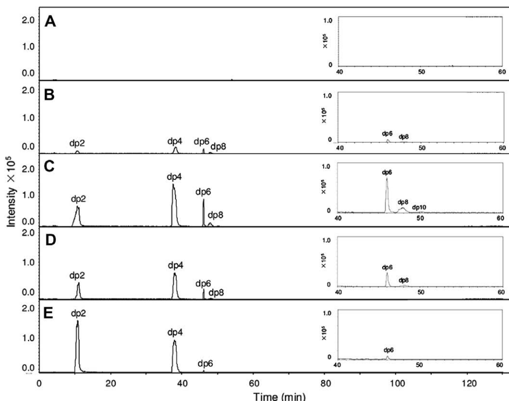
Fig. 7. EIC of products digested by chondroitinase AC ( F. heparinum ): (A) 0-min aliquots; (B) 10-min aliquots; (C) 30-min aliquots; (D) 60-min aliquots; (E) 120-min aliquots. Insets are 2.5× intensity magnification of 40 to 60 min.
